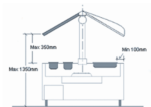
Figure 5: Examples of approved sneeze guards or protective barriers on salad bars and food preparation bench
