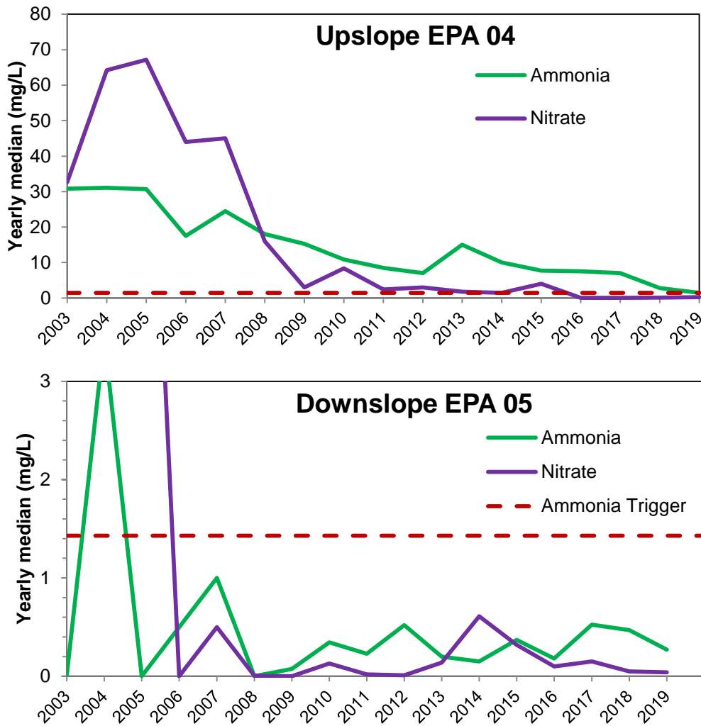
Figure 3-1: Yearly median Ammonia and Nitrate values at alluvial groundwater bores (EPA 04 upslope and EPA 05 downslope)
