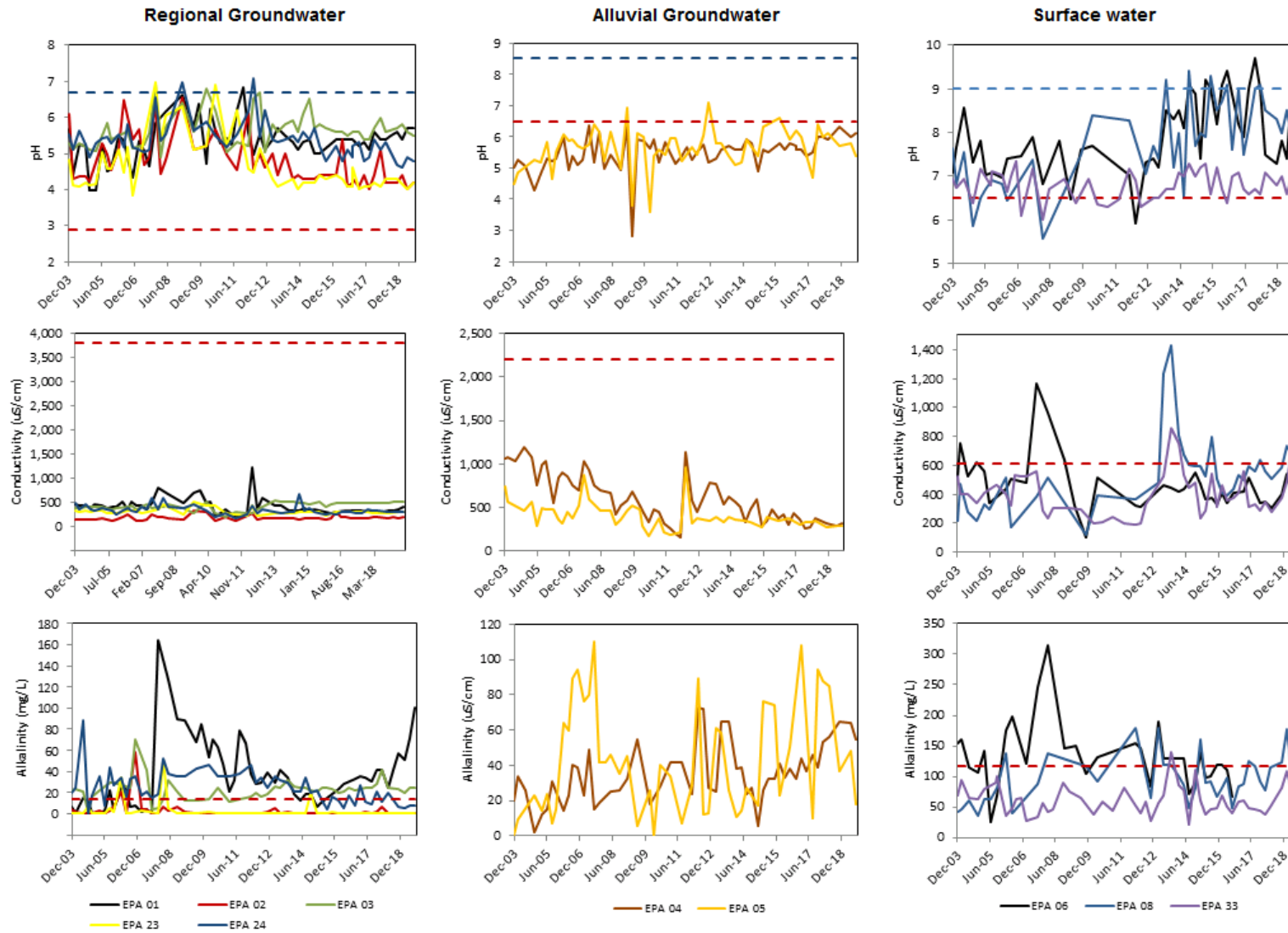
Figure 3-7: Regional Groundwater, Alluvial Groundwater and Surface water monitoring results between 2003 and 2019
