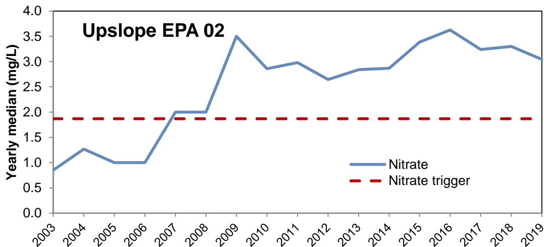
Figure 3-3: Increase in Nitrate within monitoring bore EPA 02
