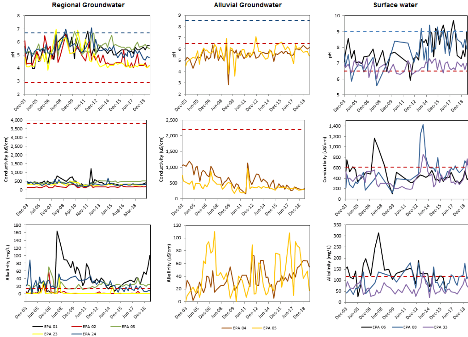
Figure 3-8: Regional Groundwater, Alluvial Groundwater and Surface water monitoring results between 2003 and 2019
