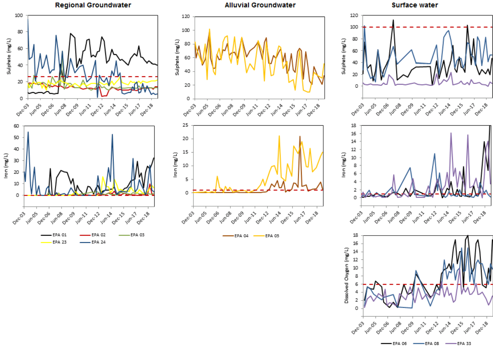
Figure 3-11: Regional Groundwater, Alluvial Groundwater and Surface water monitoring results between 2003 and 2019
