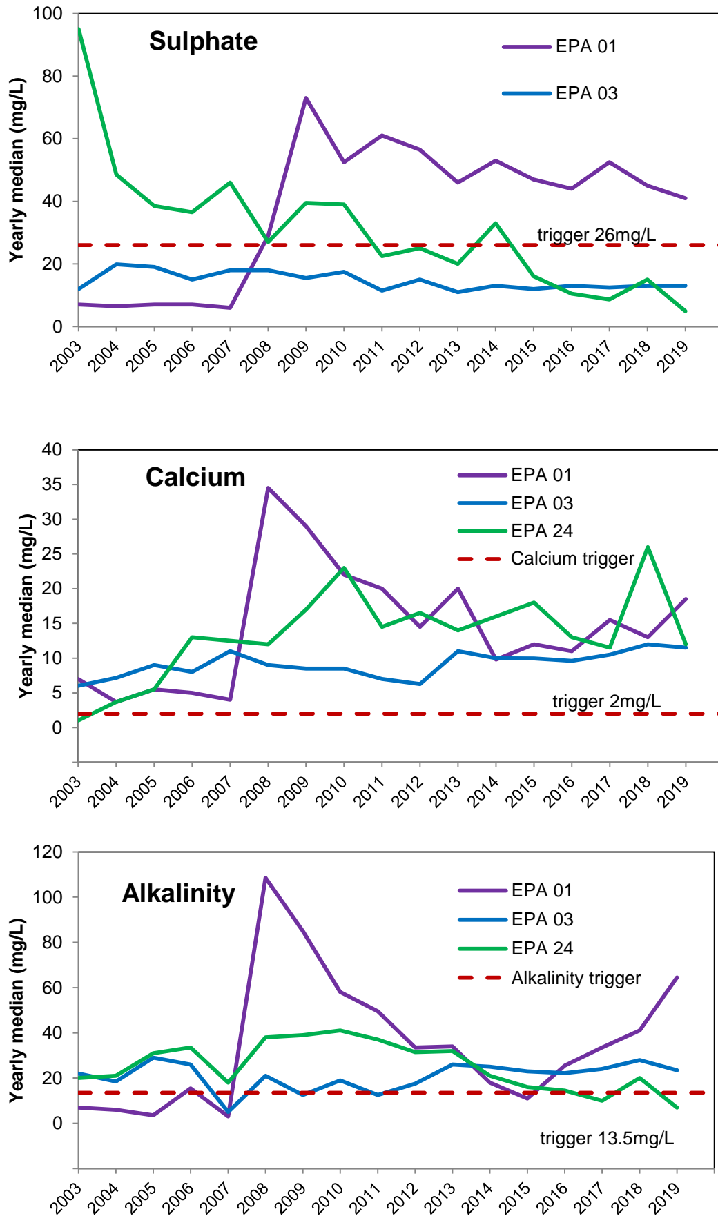
Figure 3-4: Select analytes yearly median results from downslope monitoring bores of the Regional Aquifer
