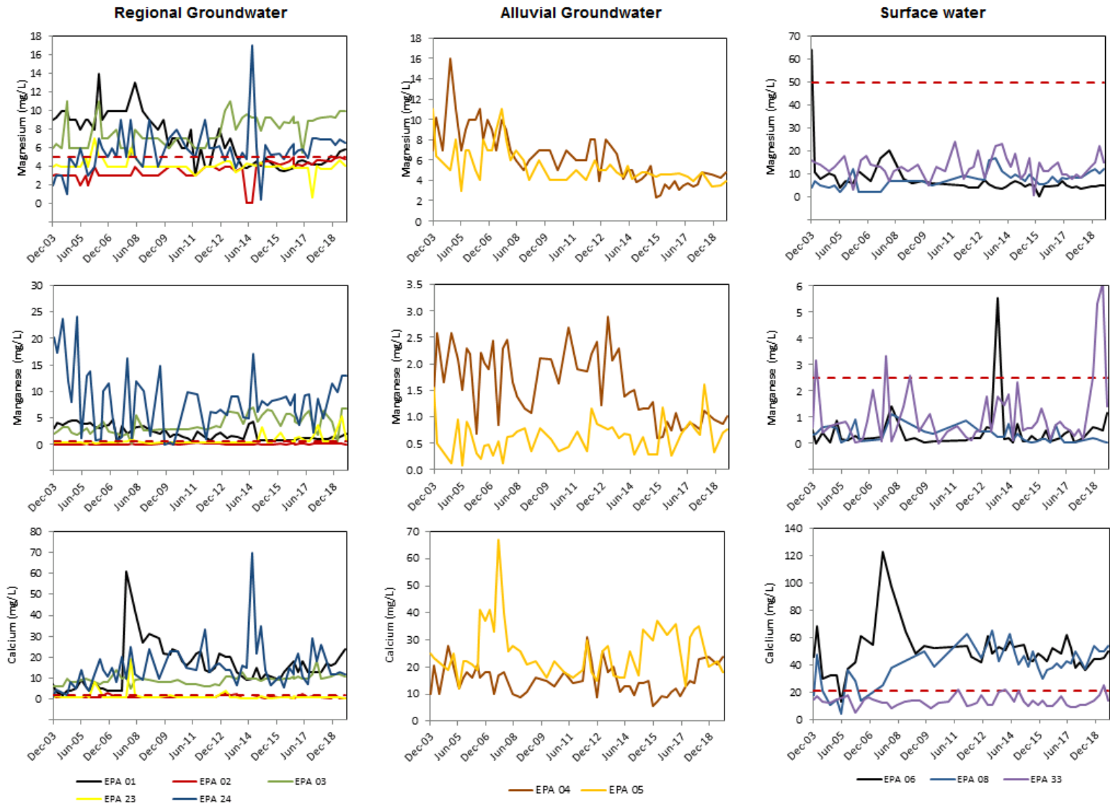
Figure 3-10: Regional Groundwater, Alluvial Groundwater and Surface water monitoring results between 2003 and 2019
