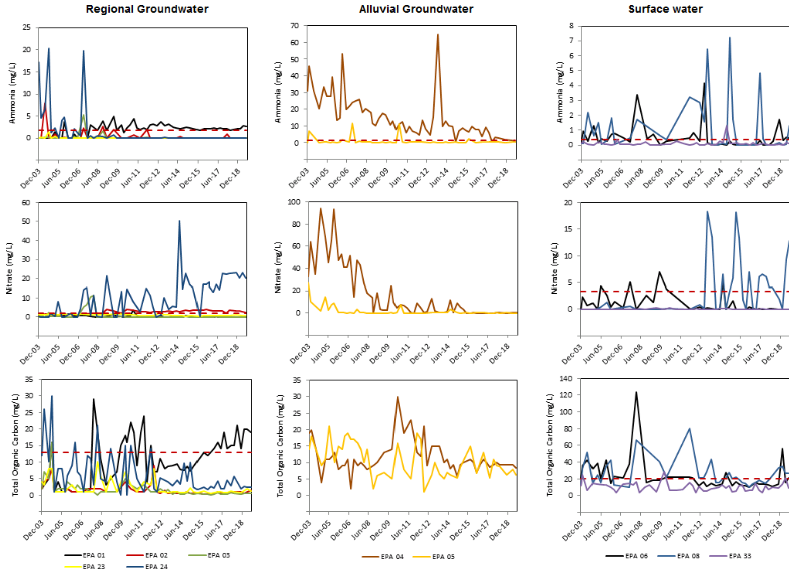
Figure 3-9: Regional Groundwater, Alluvial Groundwater and Surface water monitoring results between 2003 and 2019
