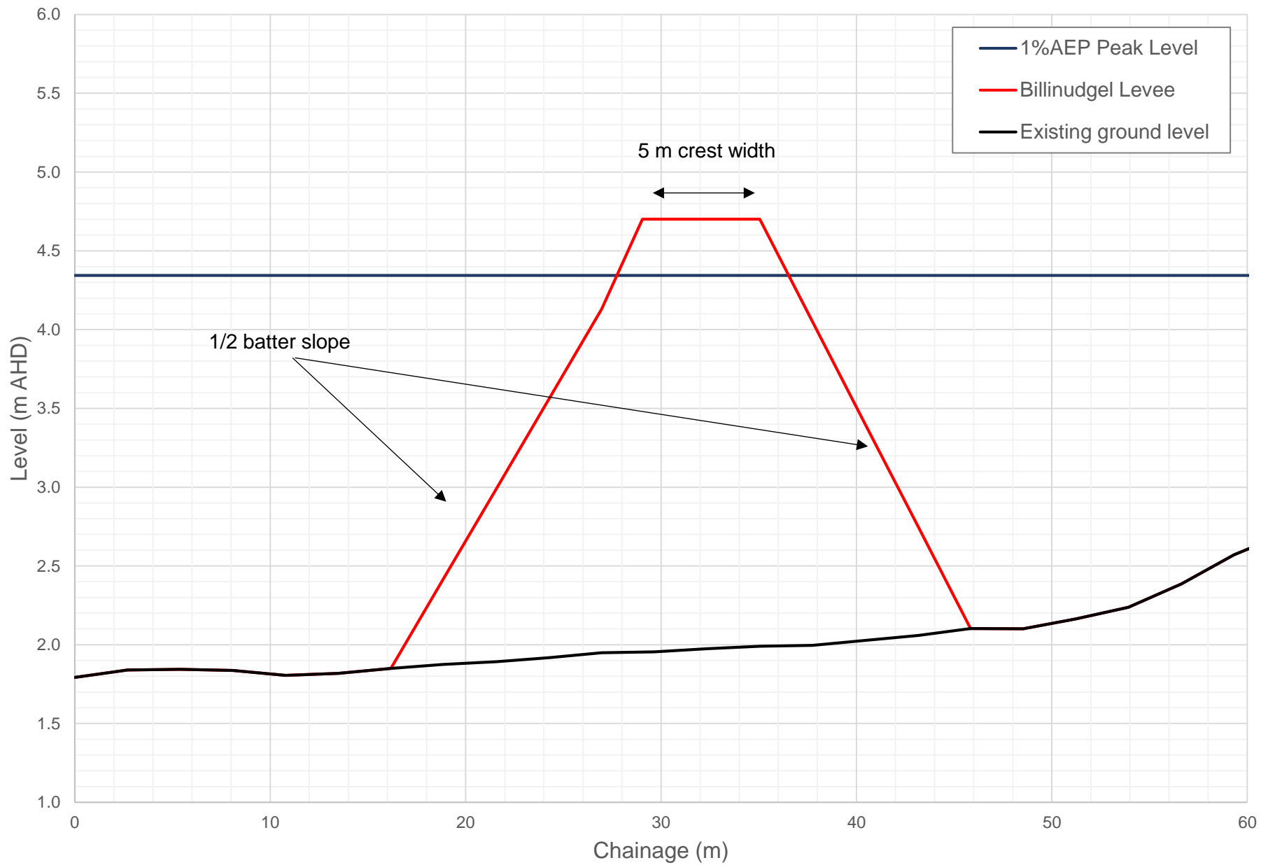
FIGURE L-2 BILLINUDGEL MITIGATION OPTION TYPICAL LEVEL CROSS SECTION
