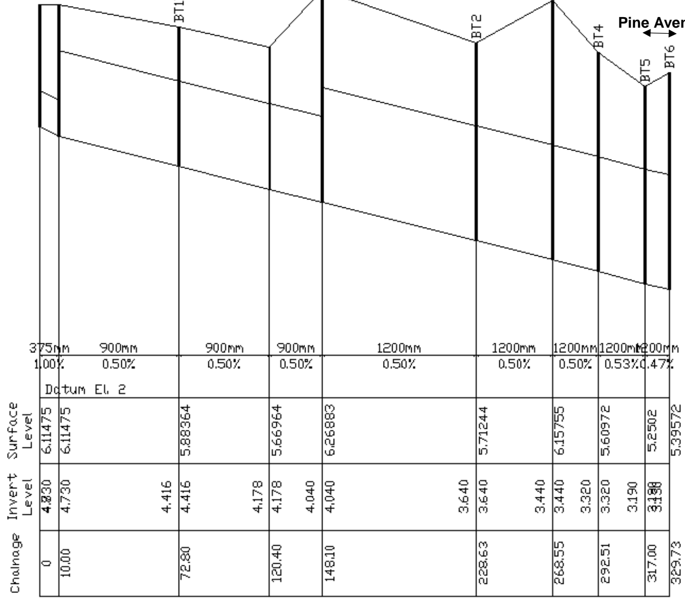
AVOCADO COURT AND GREVILLEA AVENUE MITIGATION OPTION LONG SECTION
