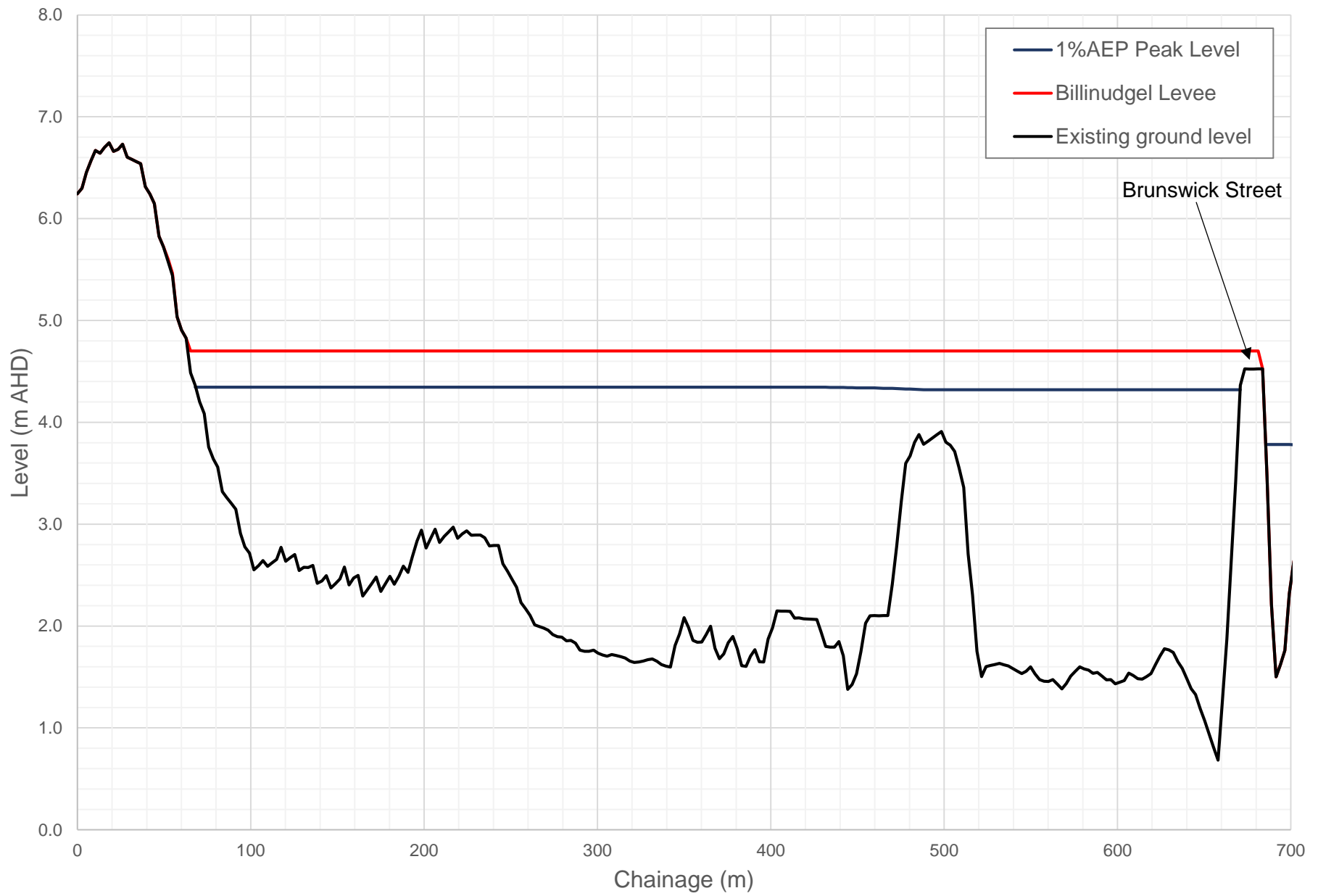
FIGURE L-1 BILLINUDGEL MITIGATION OPTION LEVEL LONG PROFILE
