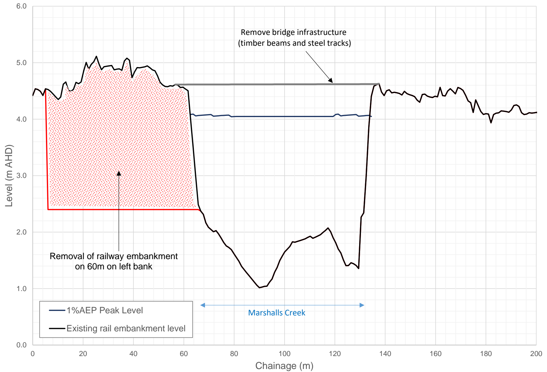
LEFT BANK RAIL EMBANKMENT REMOVAL AT MARSHALLS CREEK BILLINGDEL MITIGATION OPTION FIGURE L-3
