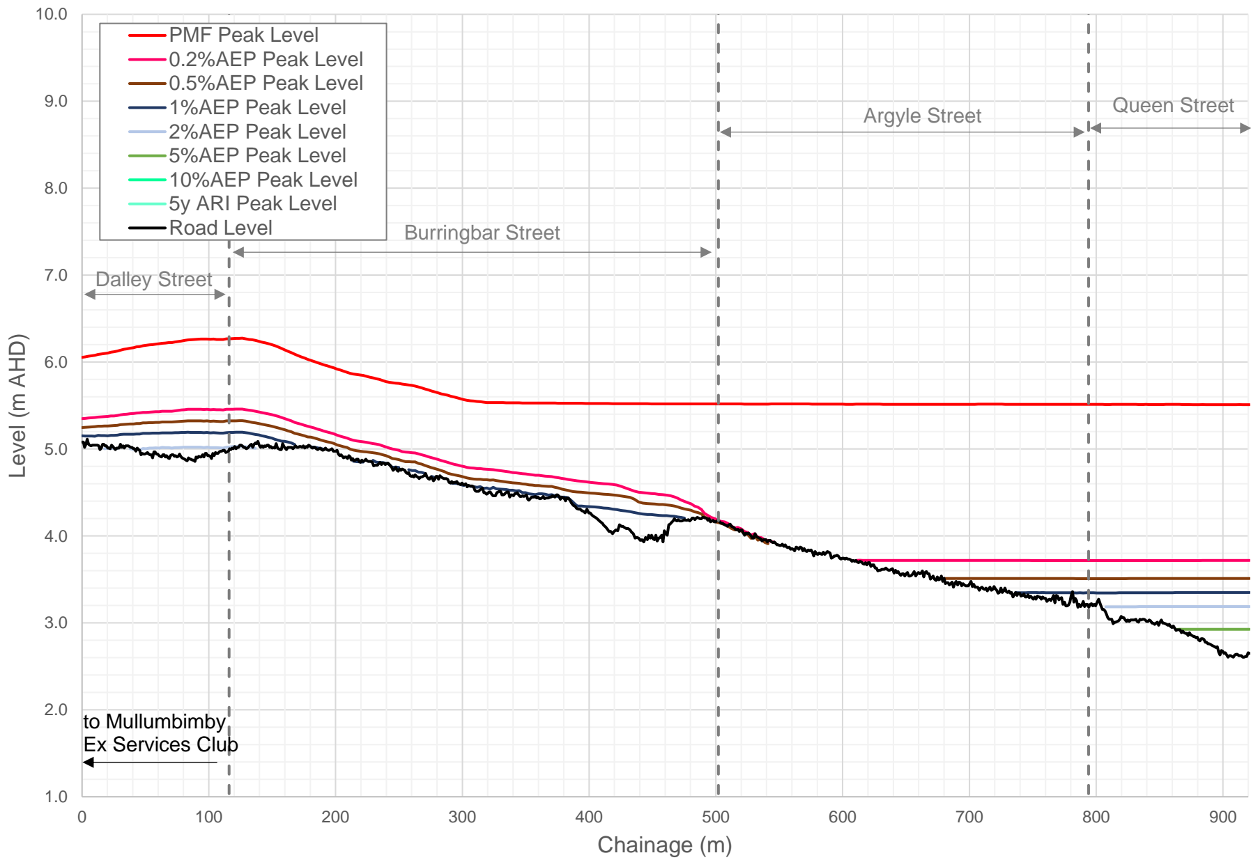
FIGURE J4 LONG PROFILE MULLUMBIMBY EAST EVACUATION ROUTE
