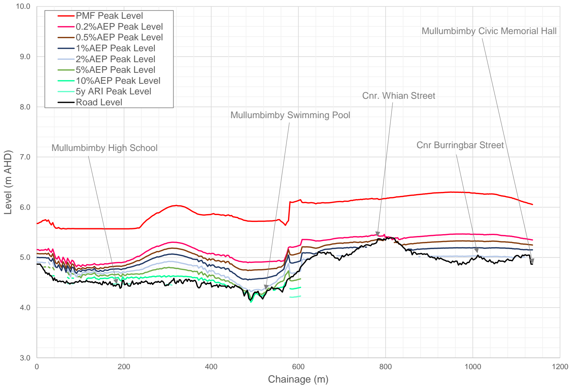
FIGURE J8 LONG PROFILE MULLUMBIMBY SOUTH EVACUATION ROUTE
