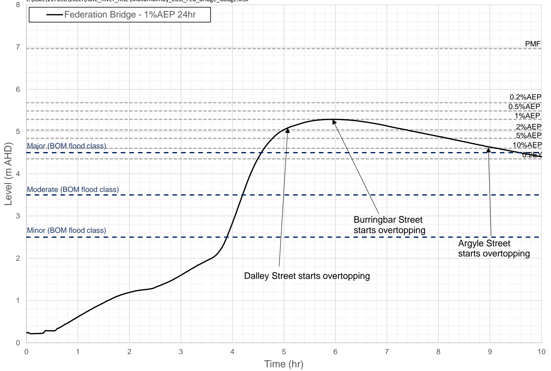
1% AEP DESIGN EVENT - EVACUATION ROUTE MULLUMBIMBY EAST STAGE HYDROGRAPH AT FEDERATION BRIDGE GAUGE FIGURE J3
