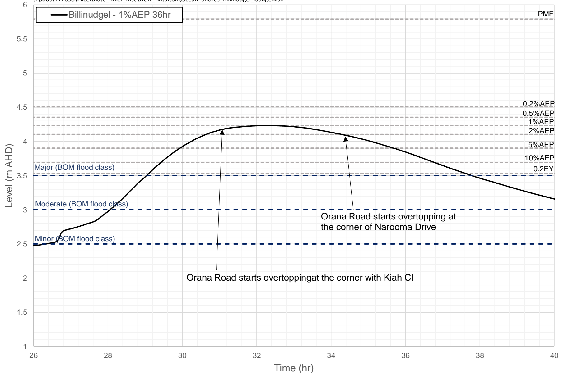
FIGURE J11 1% AEP DESIGN EVENT - EVACUATION ROUTE OCEAN SHORES STAGE HYDROGRAPH AT BILLINUDGEL GAUGE
