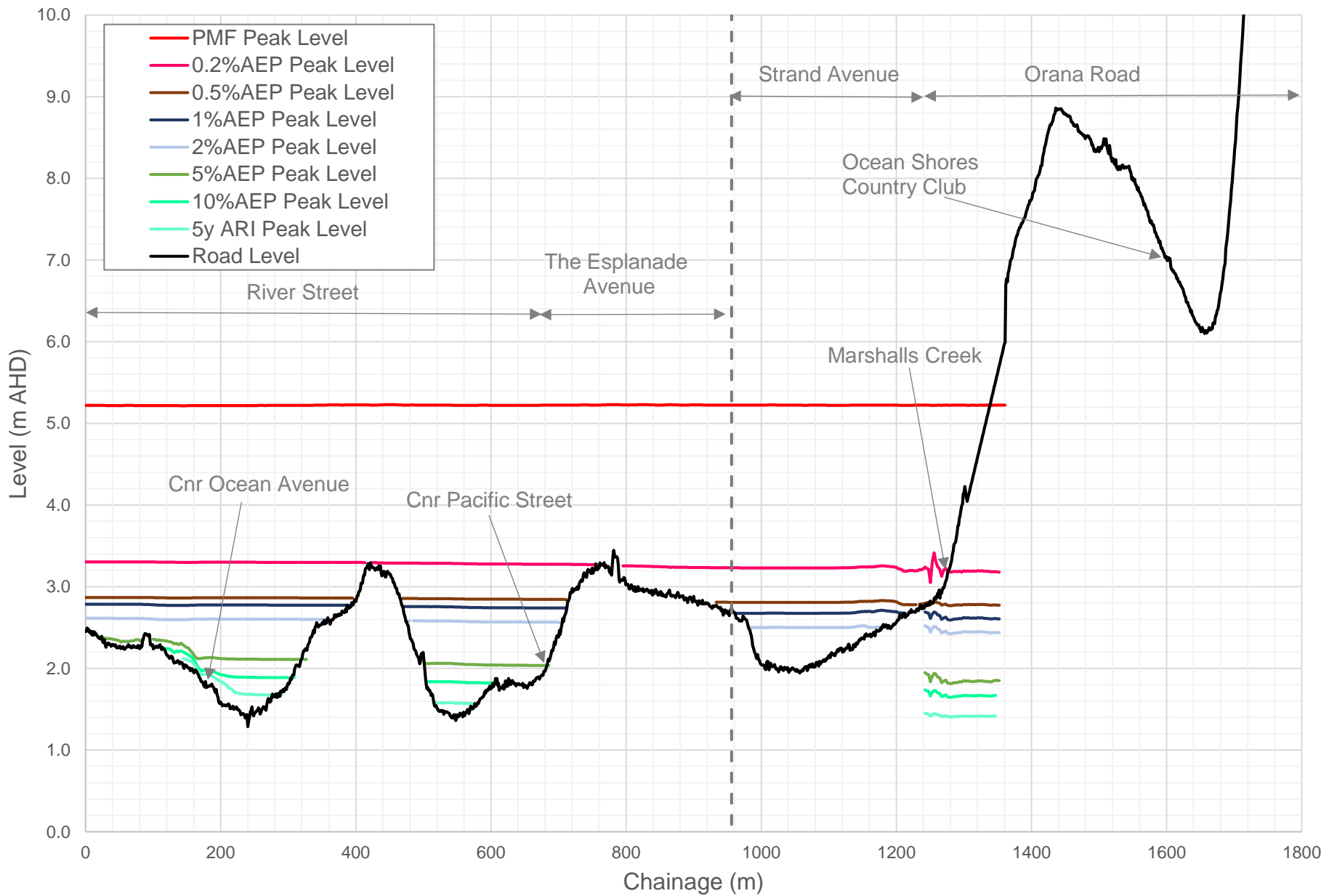
FIGURE J10 LONG PROFILE NEW BRIGHTON AND OCEAN SHORES EVACUATION ROUTE
