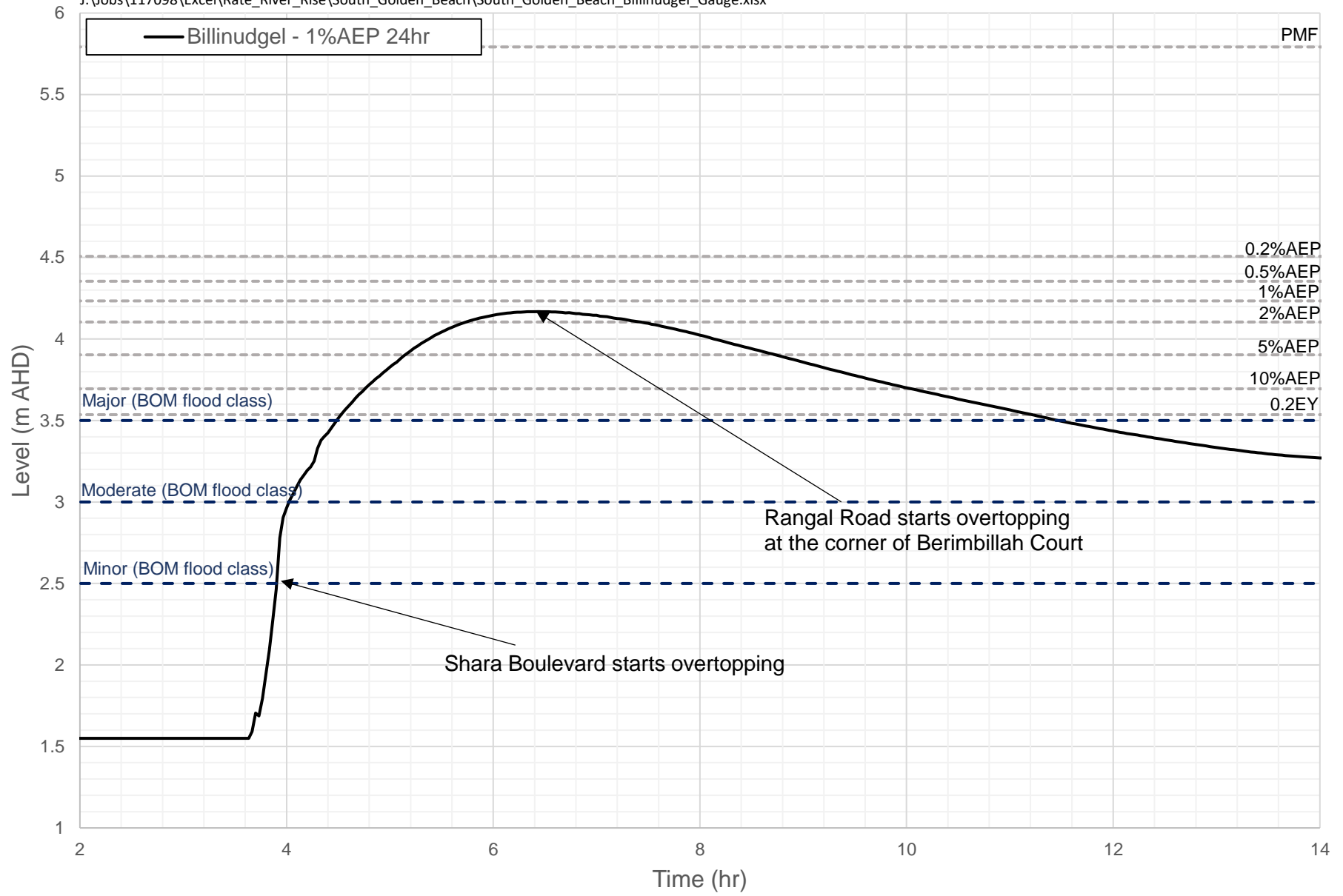
FIGURE J13 1%AEP DESIGN EVENT - EVACUATION ROUTE SOUTH GOLDEN BEACH STAGE HYDROGRAPH AT BILLINUDGEL GAUGE
