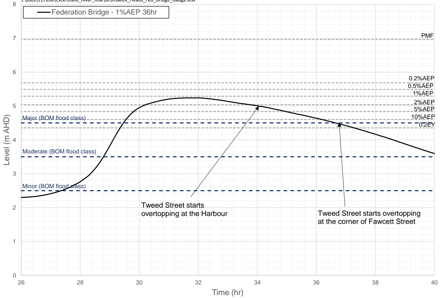
1%AEP DESIGN EVENT - EVACUATION ROUTE BRUNSWICK HEADS STAGE HYDROGRAPH AT FEDERATION BRIDGE GAUGE FIGURE J1
