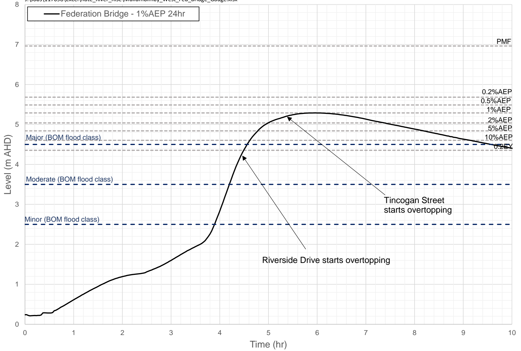
1%AEP DESIGN EVENT - EVACUATION ROUTE MULLUMBIMBY WEST STAGE HYDROGRAPH AT FEDERATION BRIDGE GAUGE FIGURE J5
