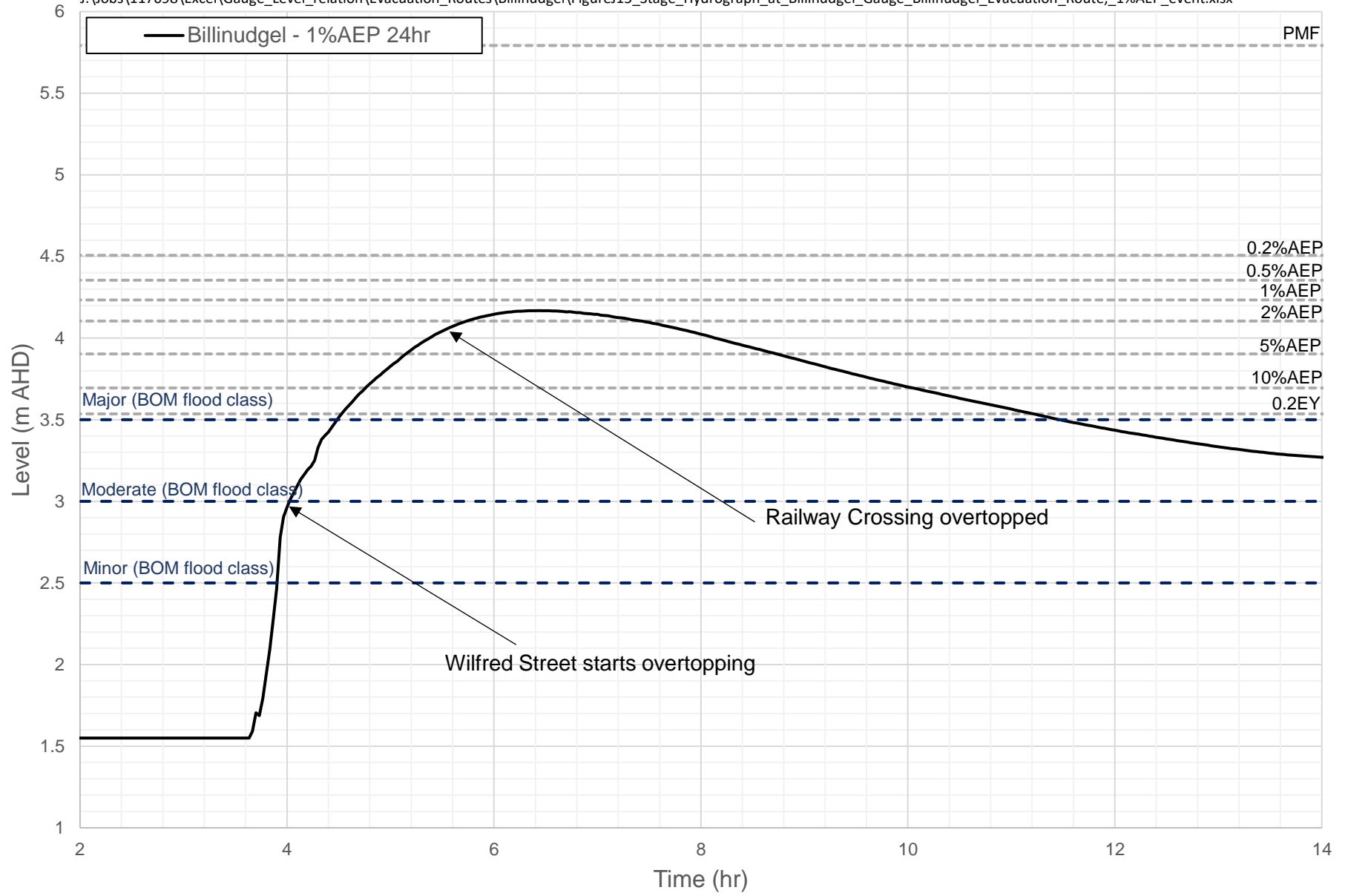
FIGURE J15 1%AEP DESIGN EVENT - EVACUATION ROUTE BILLINUDGEL STAGE HYDROGRAPH AT BILLINUDGEL GAUGE
