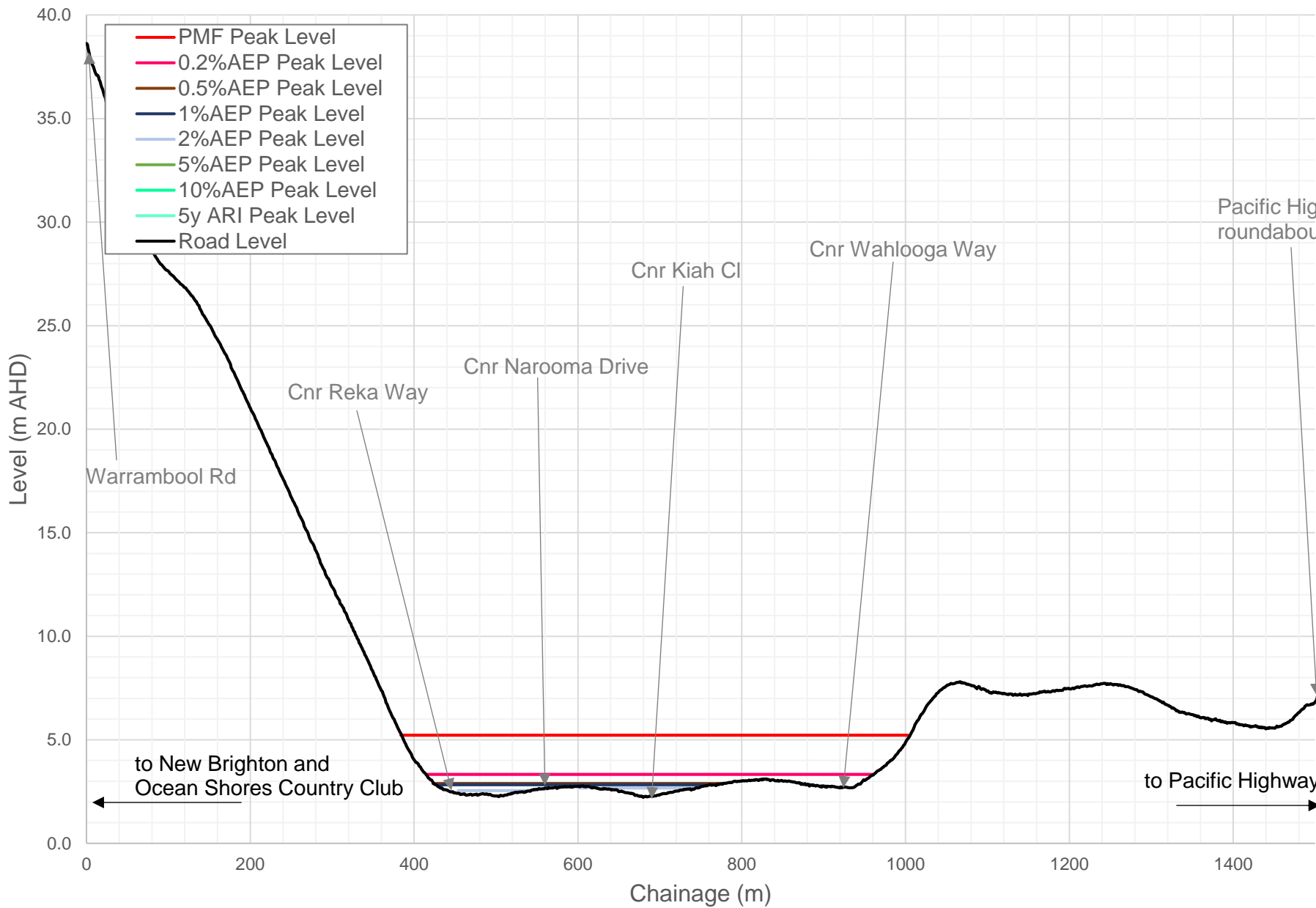
FIGURE J12 LONG PROFILE OCEAN SHORES ORANA ROAD EVACUATION ROUTE
