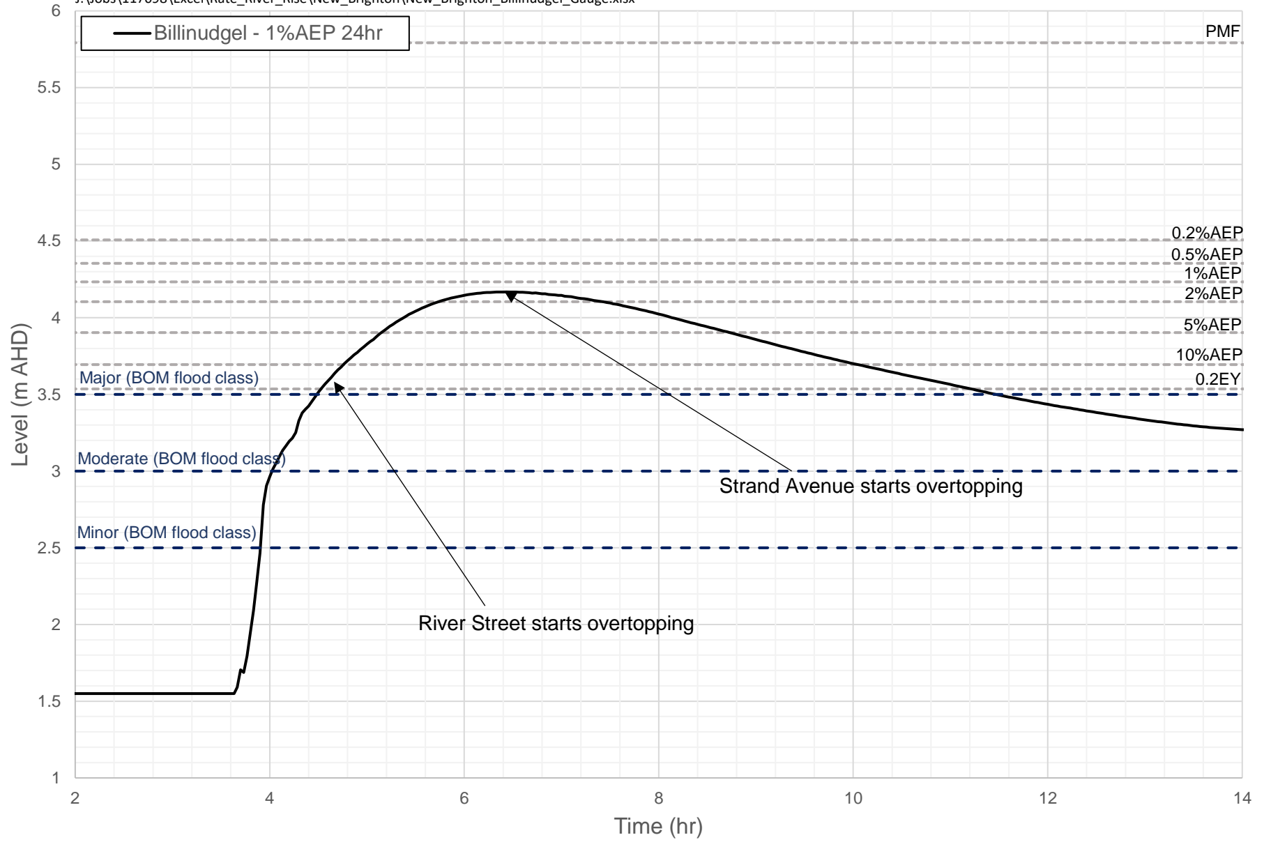
1%AEP DESIGN EVENT - EVACUATION ROUTE NEW BRIGHTON STAGE HYDROGRAPH AT BILLINUDGEL GAUGE FIGURE J9
