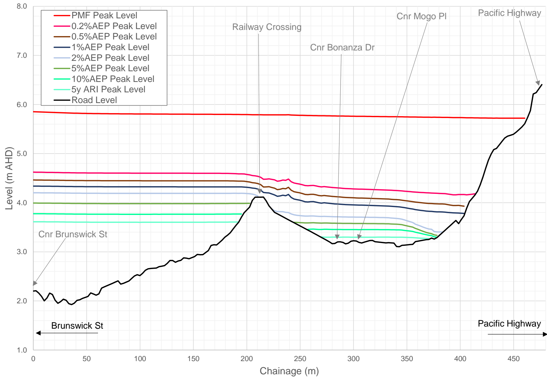
BILLINUGDEL WILFRED STREET EVACUATION ROUTE LONG PROFILE FIGURE J16
