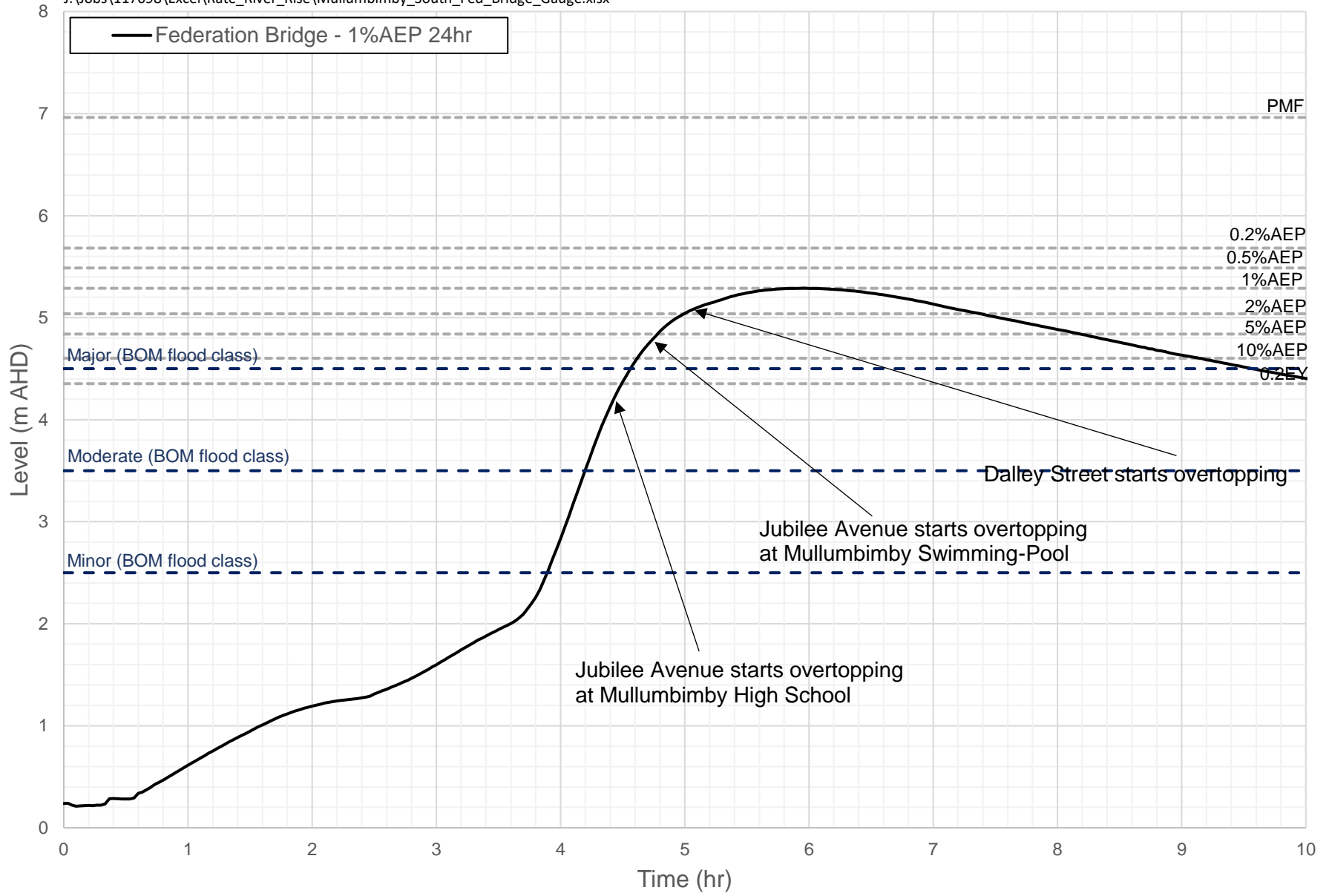
1%AEP DESIGN EVENT - EVACUATION ROUTE MULLUMBIMBY SOUTH STAGE HYDROGRAPH AT FEDERATION BRIDGE GAUGE FIGURE J7
