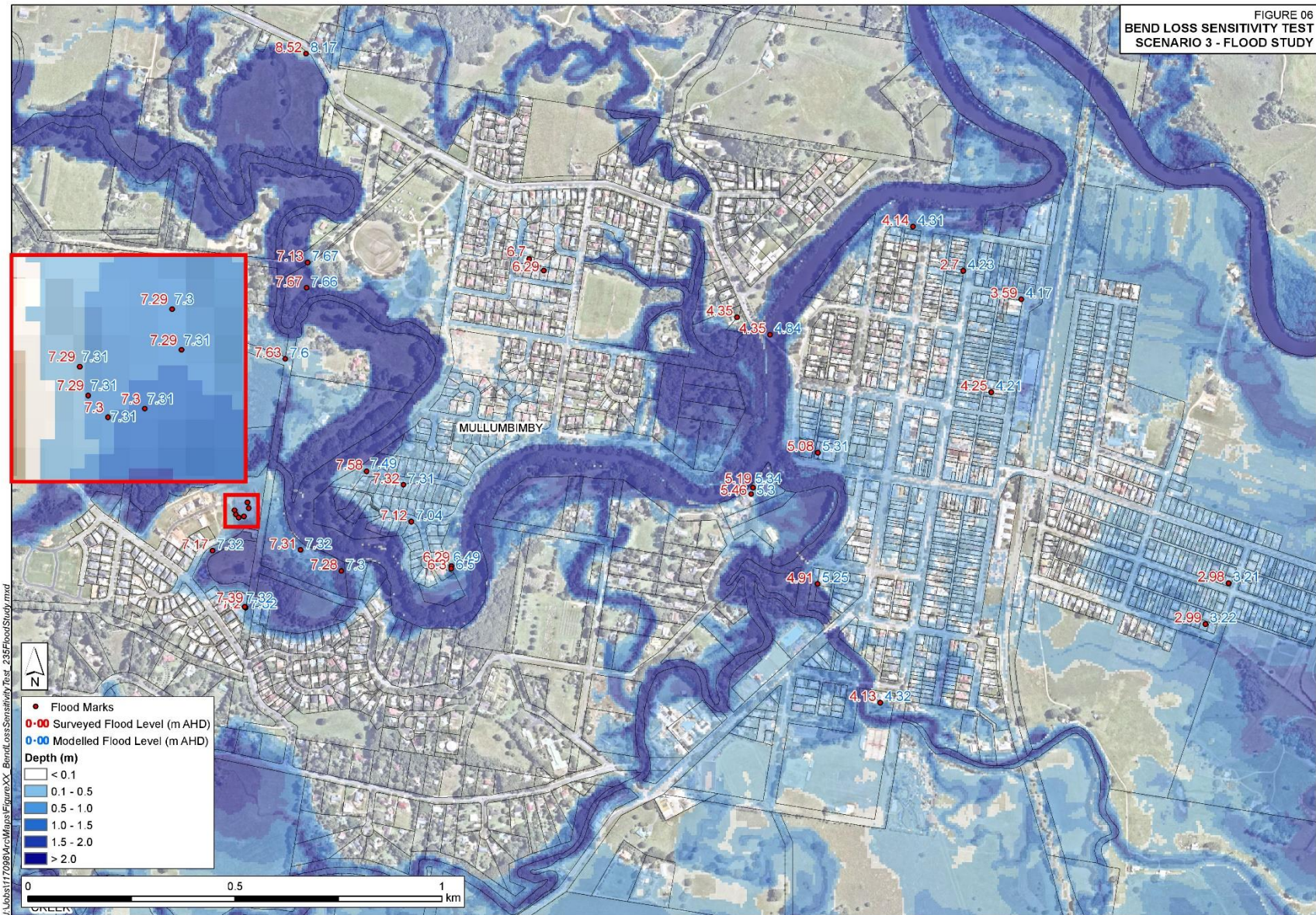
Figure E6: Calibration Results – March 2017 event using Scenario 3 bend losses
