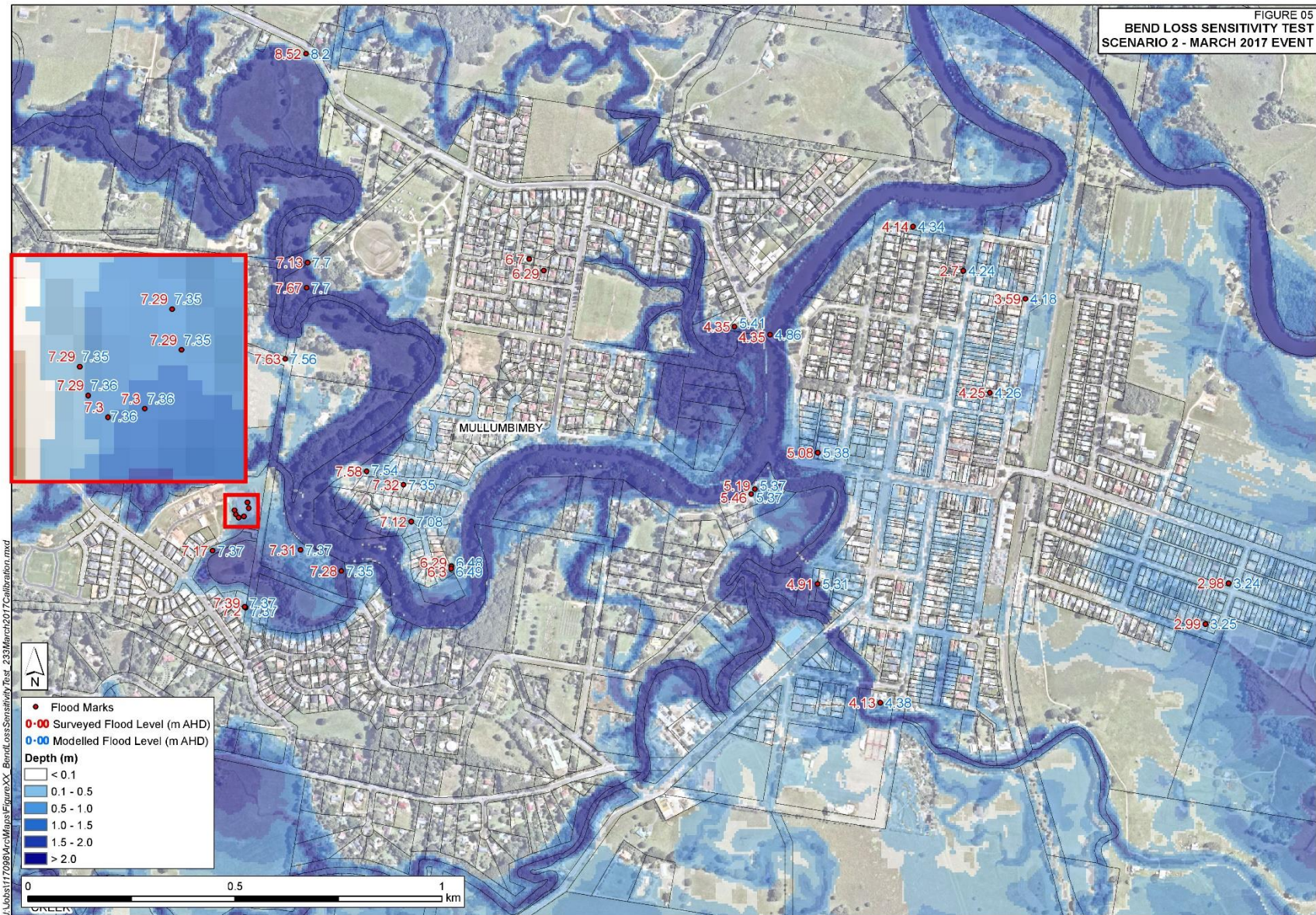
Figure E5: Calibration Results – March 2017 event using Scenario 2 bend losses
