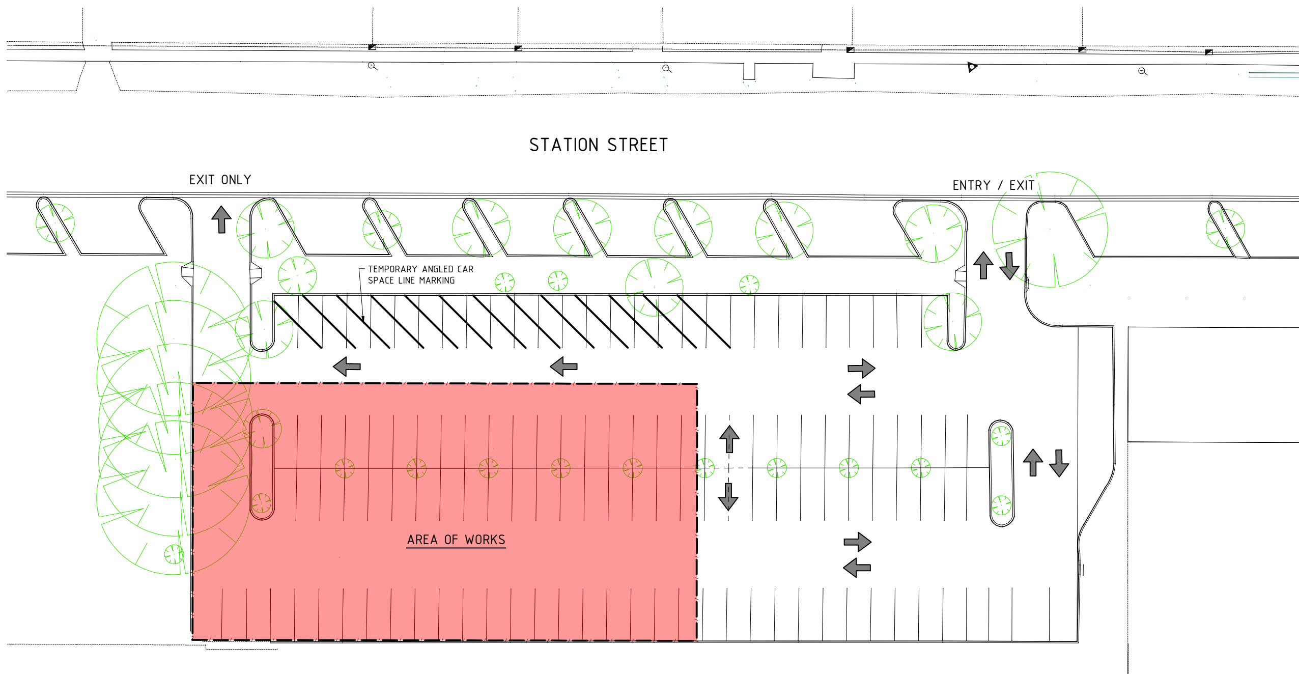
TEMPORARY CAR PARK PLAN SCALE 1:400 (A3)
